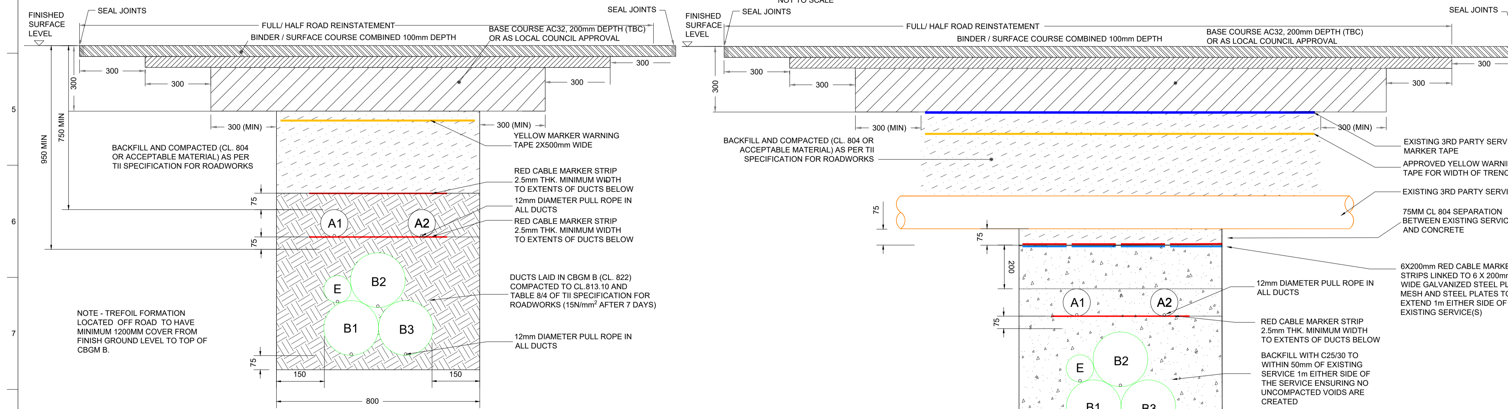
SECTION B-B TYPICAL TREFOIL CROSS SECTION INDICATING TRENCH FOR 220KV CIRCUIT UNDER ROADS
