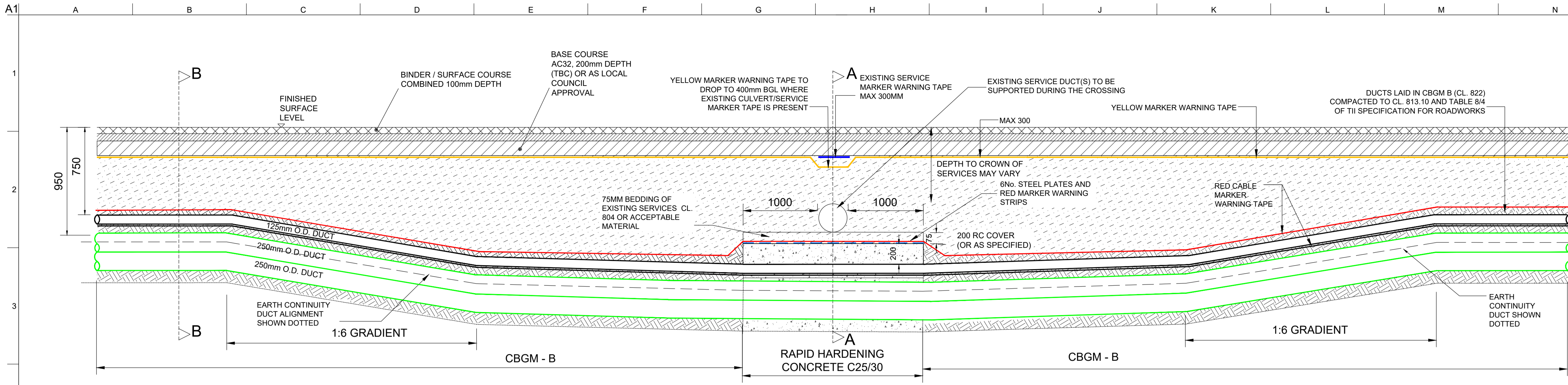
TYPICAL TREFOIL CROSS SECTION ON -ROAD UNDER 3RD PARTY SERVICE
